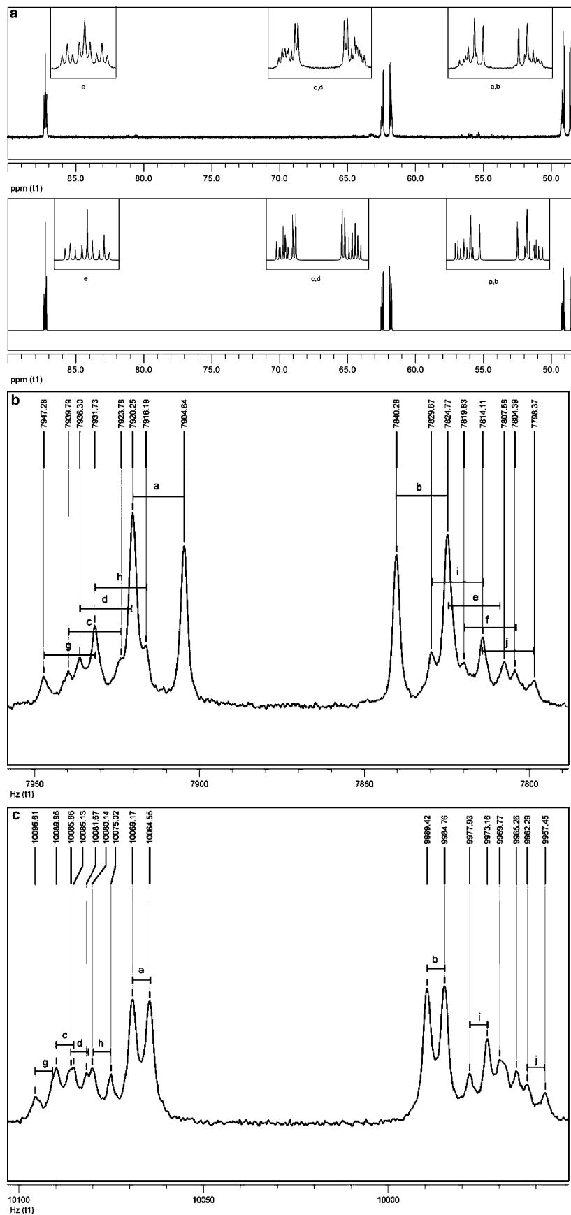
Figure 4. (a) ^{31}P\{^1H\} -NMR (161.98 MHz, in THF- d_8 ) of [Mo(N_2)(dpepp)(depe)] ( 1 ), measured (top) and simulated (bottom); (b) M-Spectrum of 1 , expansion of the signal at 48.80 ppm; (c) X-Spectrum of 1 , expansion of the signal at 62.12 ppm.
